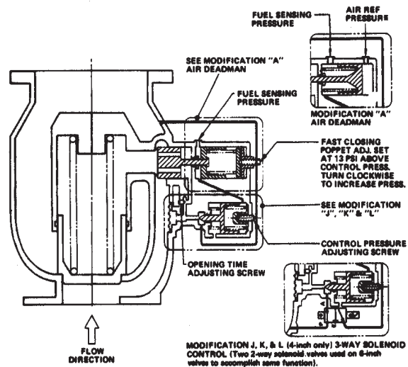
Functional schematic
